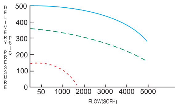
Model 330 Liquid Cylinder Regulator
